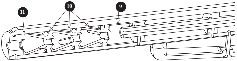
Installation of spacer, baffles and spring washer.
